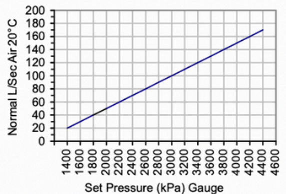
FLOW RATE CHART
