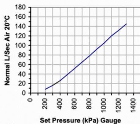
FLOW RATE CHART
